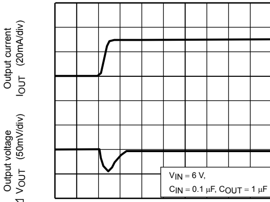
TCR5SB50U ( I_{OUT} = 1\text{m to }30\text{mA} )
