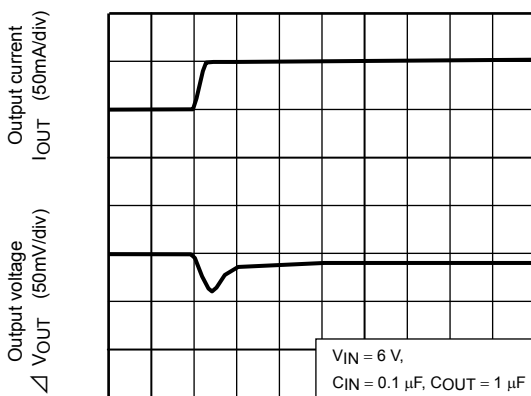
TCR5SB50U ( I_{OUT} = 50\text{m to }100\text{mA} )
