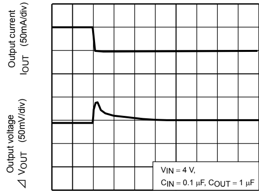
TCR5SB30U ( I_{OUT} = 100\text{m to }50\text{mA} )
