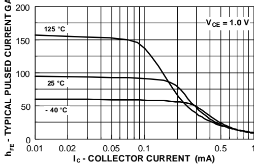
Typical Pulsed Current Gain vs Collector Current
