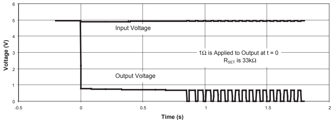
Figure 1: Overload Operation.
