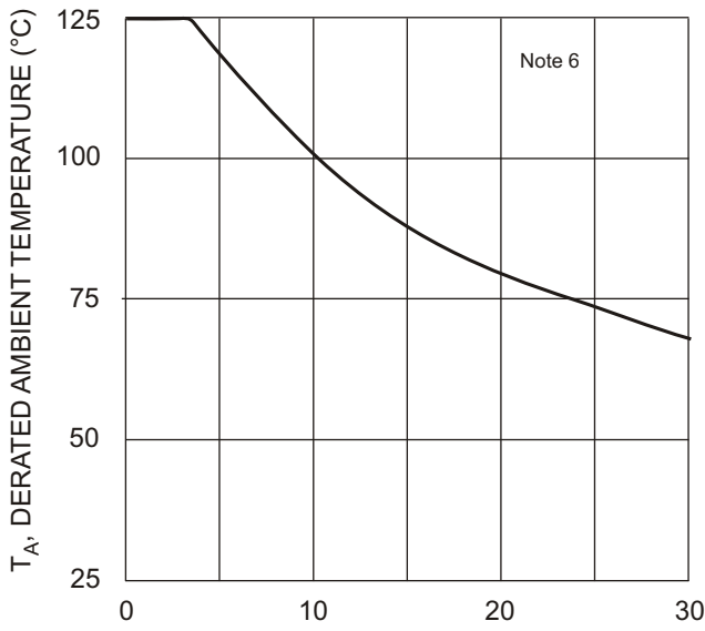
V_R , REVERSE VOLTAGE (V) Fig. 7 Operating Temperature Derating
