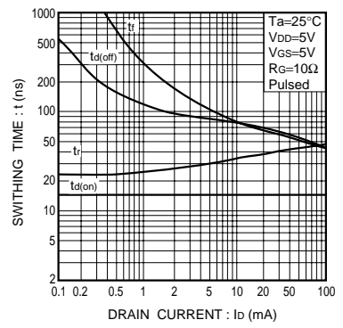
Fig.20 Switching characteristics
